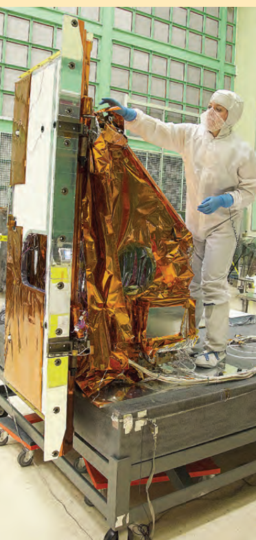
A technician reaches across the instrument to affix the corners of a multi-layer insulation blanket to the TIRS instrument.
